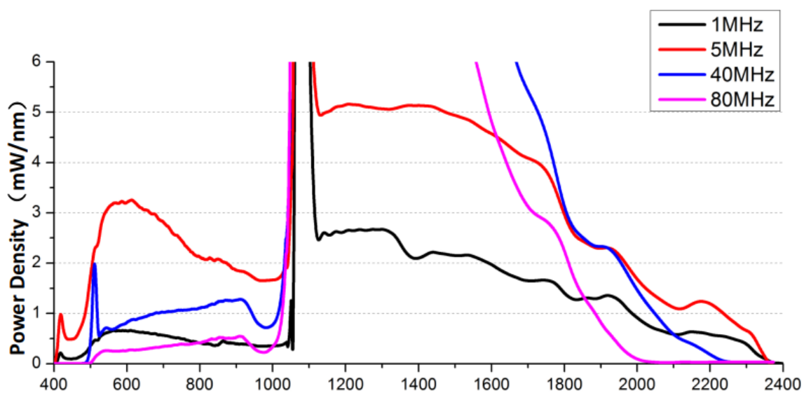
8W SC-OEM Typical Spectrum(4MHz)
